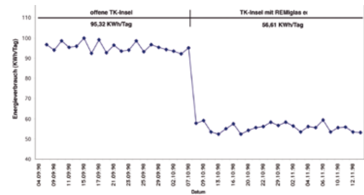
Energy consumption of the refrigerated display case
