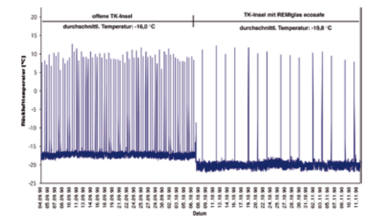
Inner temperature of the refrigerated display case
